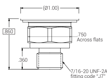
7/16-20 SAE, Male ("J7") 13.3 to 14.75 lb-ft (18-20 Nm)
