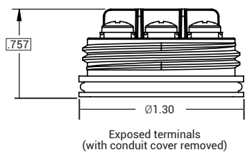
Elec. Term: 1/2" Male conduit w/ terminal strip Code: ("A1")
