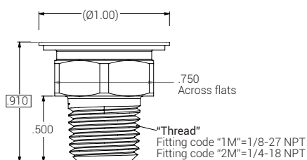
Fitting: Male NPT Code: ("1M,2M") Torque: 2-3 TFFT*
