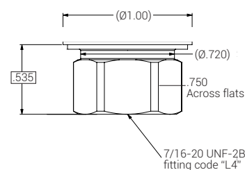
1/4 SAE, Female, 45 deg. Schrader ("L4") 13.3 to 14.75 lb-ft (18-20 Nm)
