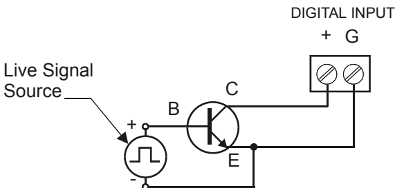
Figure 9. Digital Input From Live Signal
