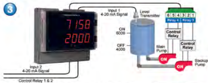
If the backup pump is not able to keep up, and the level reaches 7000 gallons, relay #4 transfers and starts the main pump as well.
