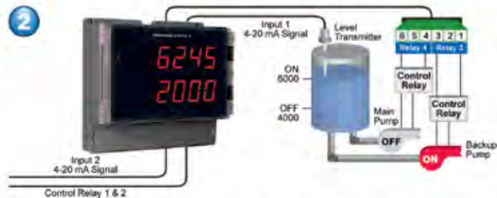
With the Pump Alternation feature activated, the next time the level reaches 6000 gallons, relay #3 transfers and starts the backup pump.
