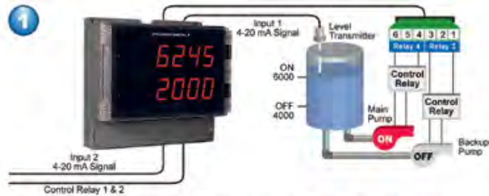
Relay #4 turns the main pump on at 6000 gallons and turns it off at 1000 gallons.
