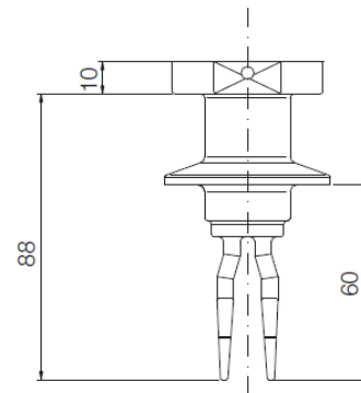
NWS-T.. Tri-clamp
