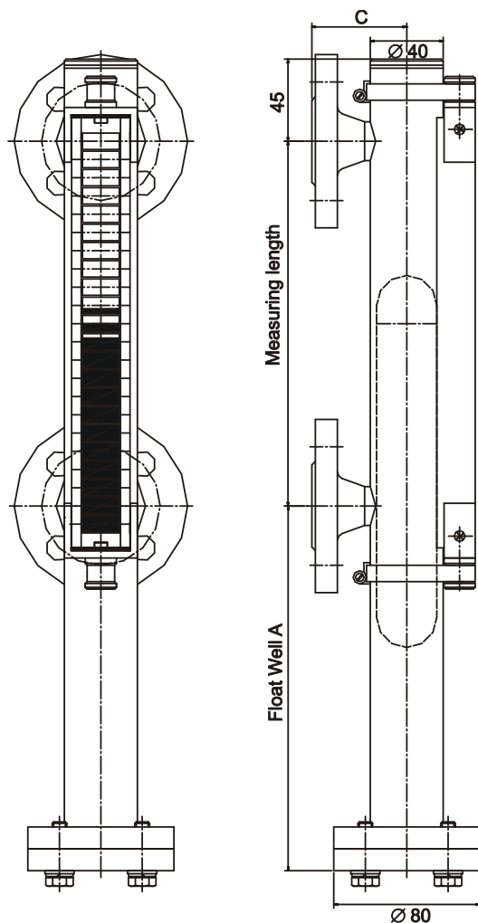
NBK-M with roller indication
