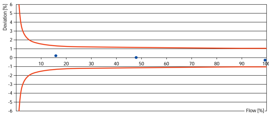
Example: Measuring points of a calibrated Truflo 5000
