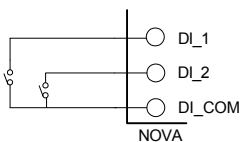
▲ Relay Contact Connection
