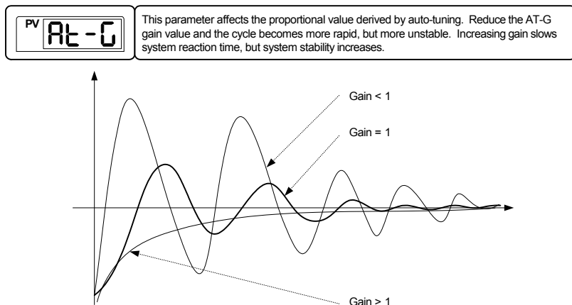
Fig 10: Auto-Tuning Gain
