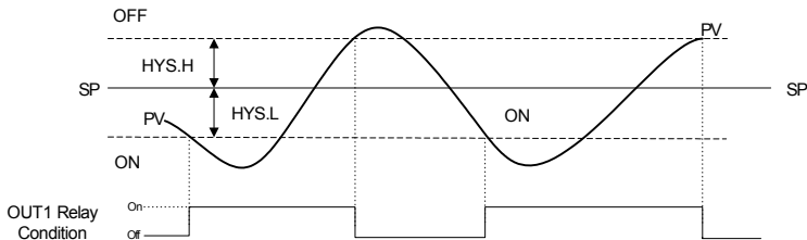
On/Off Relay Behavior Based On Hysteresis Settings
