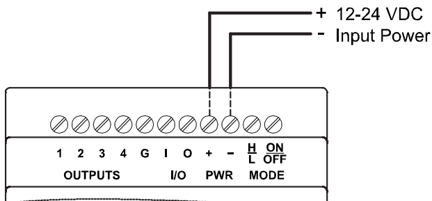
Figure 2. Power Connections
