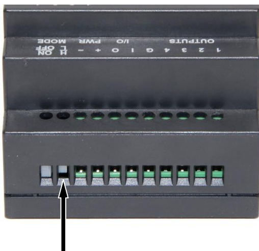
Figure 7. Inverted H/L Switch Set to Low
