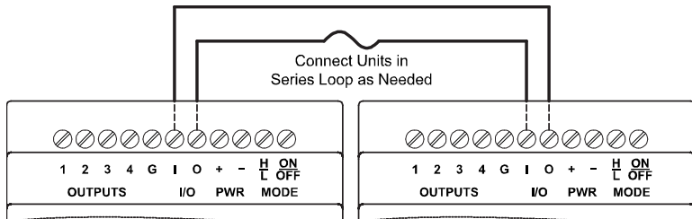
Figure 5. Cascade Mode Multiple Unit I/O Connections
