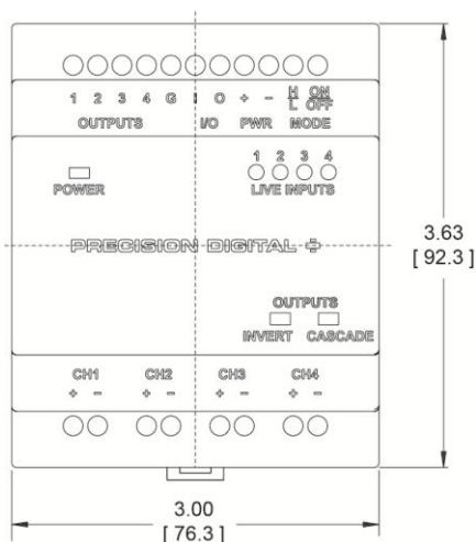
Figure 8. Dimensions - Front View
