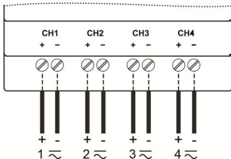
Figure 3. High Voltage Input Channel Connections
