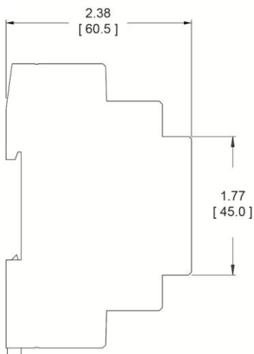
Figure 9. Dimensions - Side View
